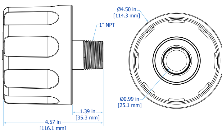
HPBT45N16-X
